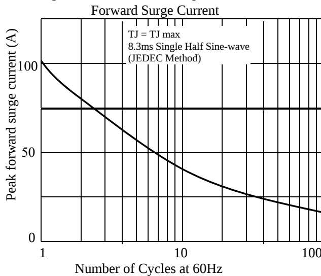
Fig. 2 - Maximum Non-repetitive Peak
