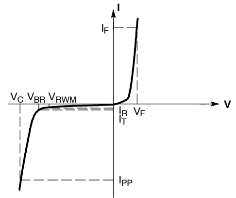
Uni-Directional TVS
