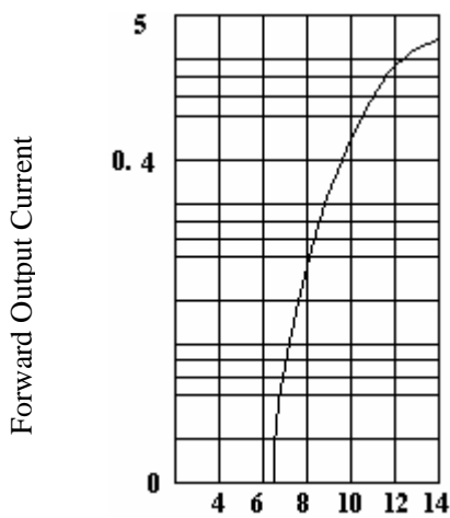
FORWARD VOLTAGE, ( V )
