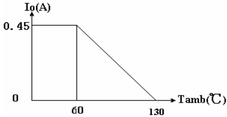
Io derating characteristic curves:
